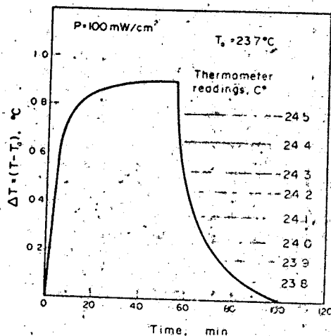
FIG. 3. The time-temperature profile for the thermistor placed in the microwave field with air as the surrounding medium is presented. Immediately after the power was terminated, a thermometer was placed at the thermistor location to check the thermistor temperature measurements.
