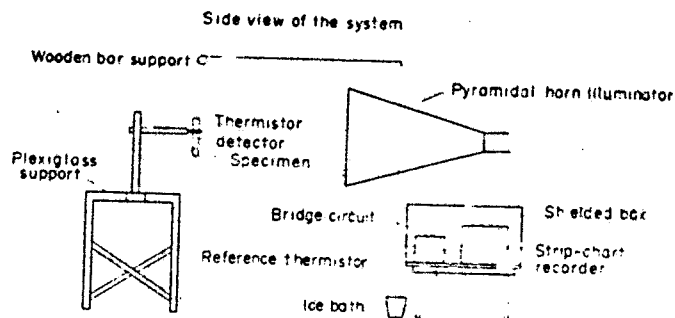
FIG. 1. Experimental exposure system consists of an absorber-lined, pyramidal horn illuminator. The specimen was a 5 ml sample of distilled water in a plastic test tube.
