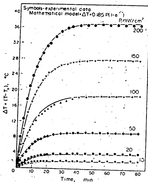
Fig. 5. Comparison of experimental and mathematical time-temperature profiles are presented. The experimental profiles are the average of four tests made on each of the exposure levels.
