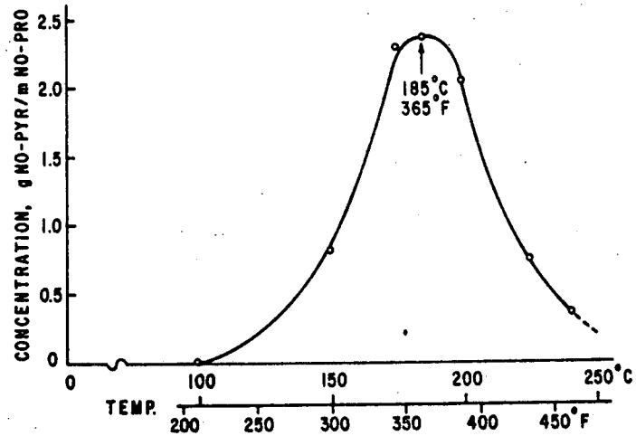
Fig. 1—Decarboxylation of nitrosoproline (NO-Pro) to nitrosopyrrolidine (NO-Pyr) in a model system.
