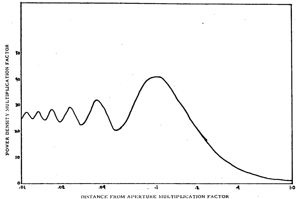
Figure 2. AXIAL POWER DENSITY IN THE NEAR FIELD NORMALIZED TO UNITY AT 2D^2/\lambda .
