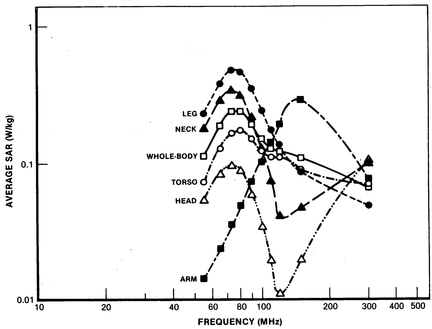
FIGURE VI-1. PARTIAL-BODY AND WHOLE-BODY AVERAGE SPECIFIC ABSORPTION RATE (SAR)* FOR A HOMOGENEOUS MODEL OF A MAN
