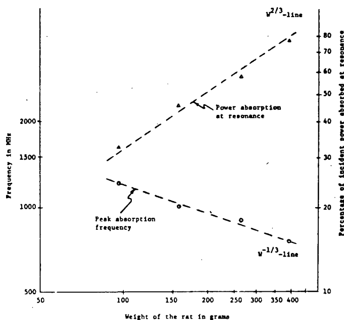
Fig. 2. Variation of the peak absorption frequency and maximum absorption with the rat weight.
