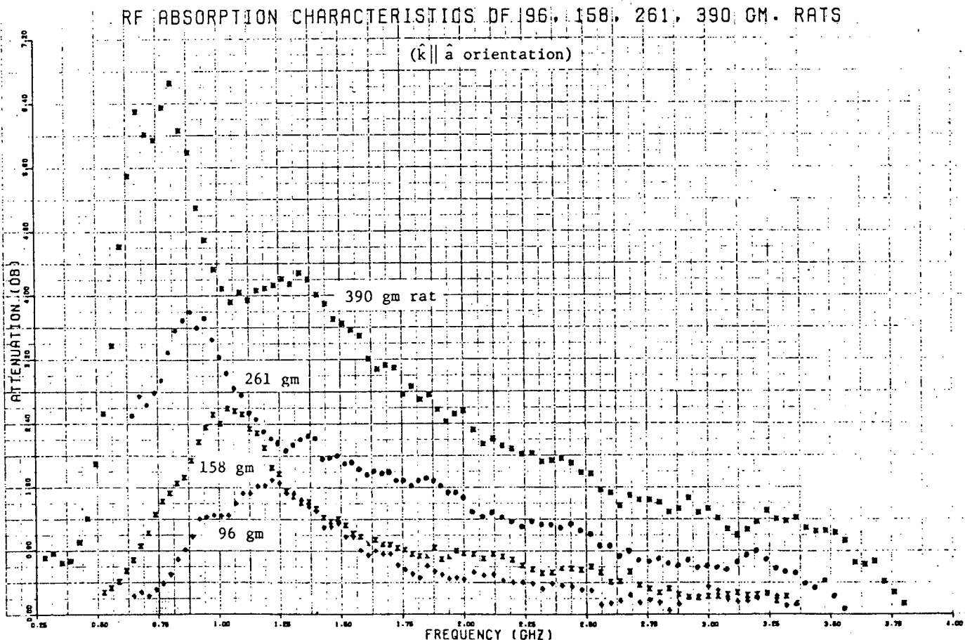
Fig. 1. RF absorption for different size rats.
