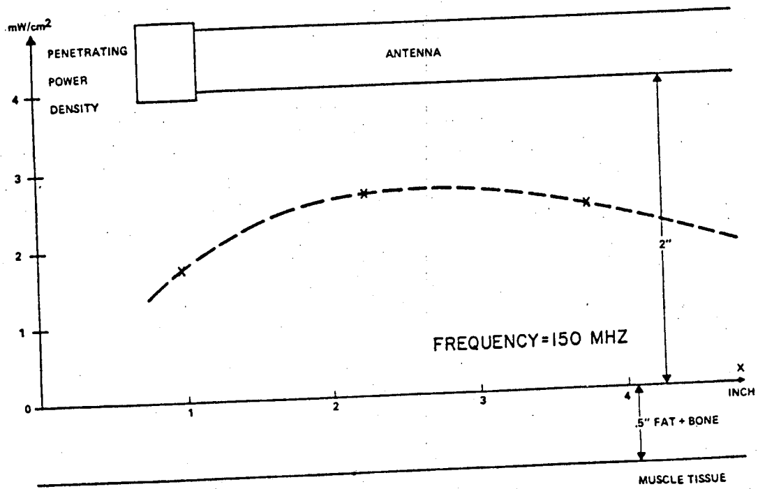
Fig. 7. Power density.
