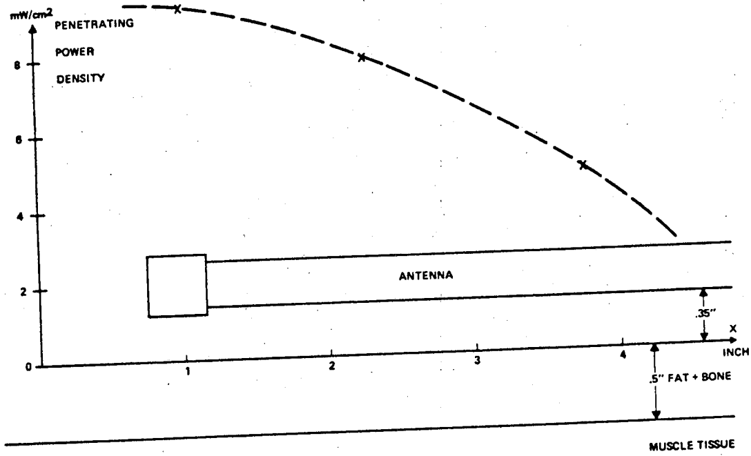
Fig. 6. Power density.
