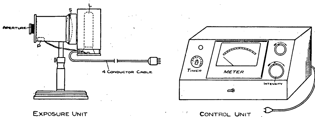
FIG. 1. SCHEMATIC DRAWING OF THE SIMPLIFIED PAIN THRESHOLD EQUIPMENT L, 500 watt lamp; S, condensing lens of 20 cm. focus; P, shutter relay.
